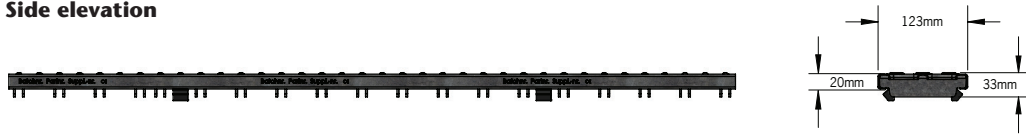
Side elevation
